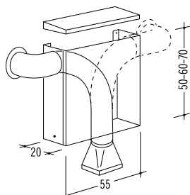
P/1F Per scarico laterale sinistro o destro Ø 15 cm For Ø 15 cm left-hand or right-hand discharge
